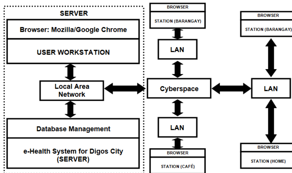
Figure 5. The System Architecture for the Digos City e-Health (Deployment Environment)
